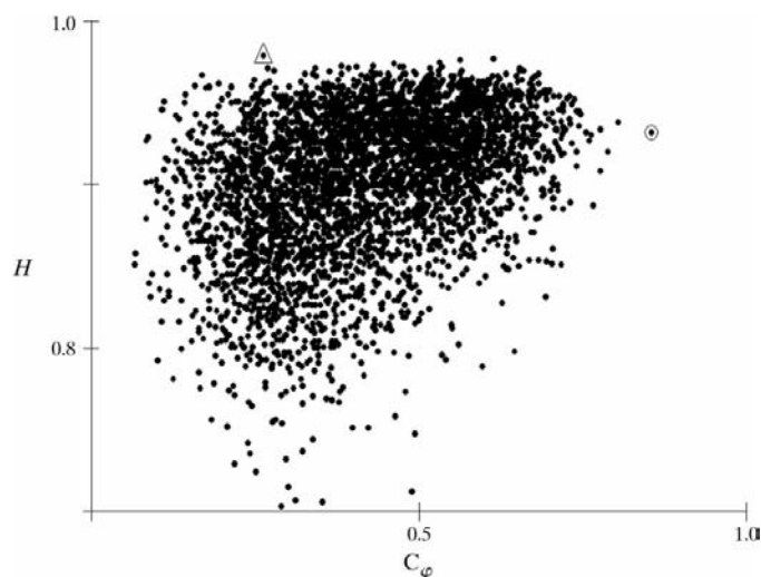
Figure 2 The analysis of 4000 randomly generated 16 Å resolution phase sets (39 independent reflections each) for RNase Sa. Every point in the diagram corresponds to one phase set and its coordinates are the map correlation coefficient C_\varphi and the histogram correlation coefficient H . The triangle marks the phase set resulting in the best histogram. The circle marks the phase set resulting in the map closest to the true one; this map cannot be identified by the H criterion.
