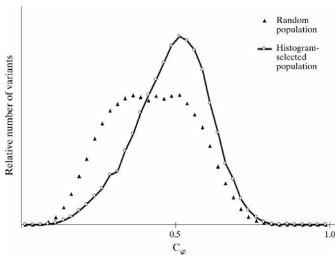
Figure 3 The distribution of the variants in the start (random) and selected populations with the map correlation coefficient (in comparison with the exact 16 Å resolution map). 4000 random and 378 histogram-selected 16 Å resolution phase sets (39 independent reflections each) are analysed for RNase Sa.
